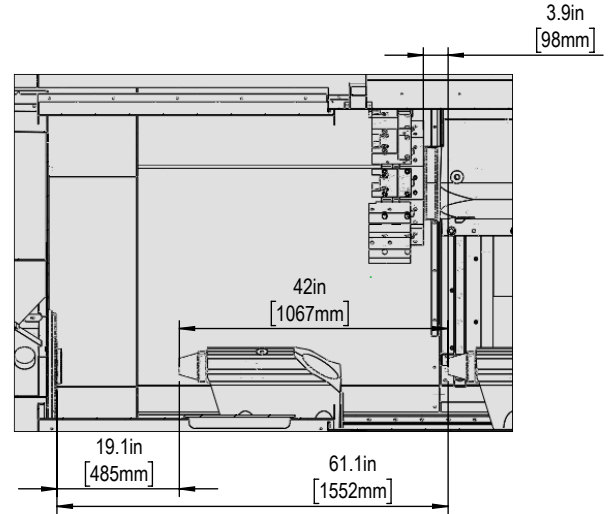
Tailstock Travels
